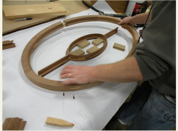
Fitting the Muntin Bar parts together
