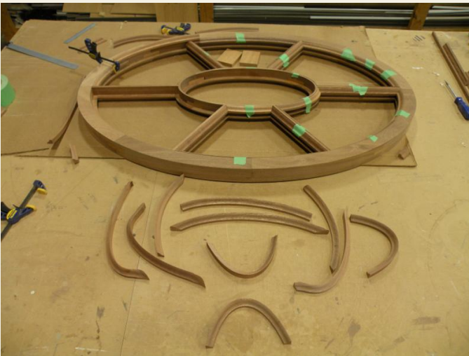
Curved Wood Glass Stop made on CNC
